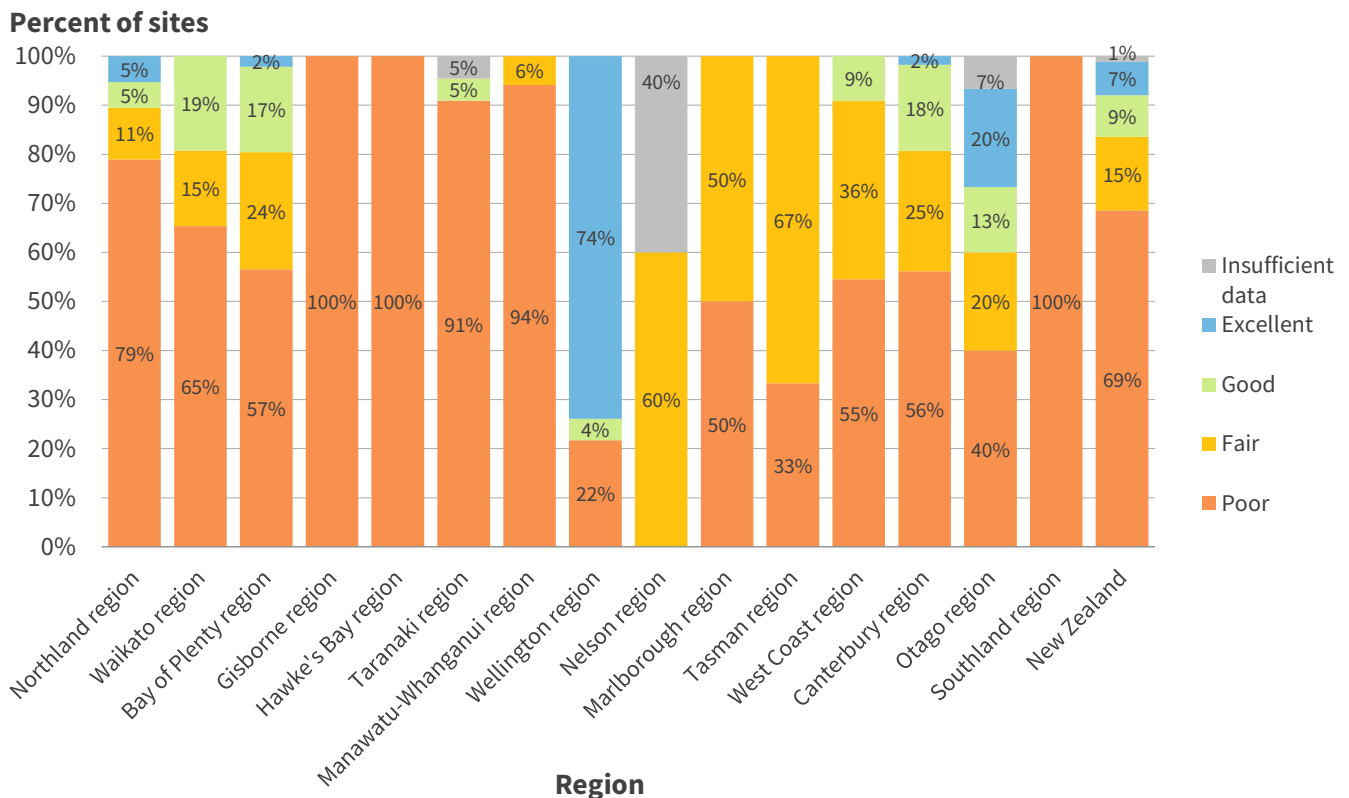
Figure 5: Bacterial risk for freshwater bathing sites, by regional council, 2018–23
